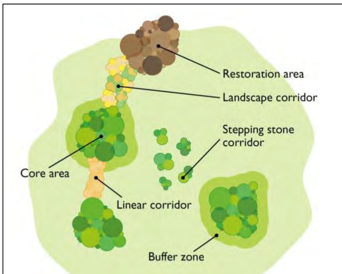
Fig 1. The Components of an Ecological Network
